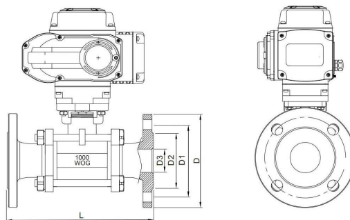
法兰型主要外形及连接法兰尺寸 GB-PN16 Flange Type Main Outline and Connecting Flange Size
